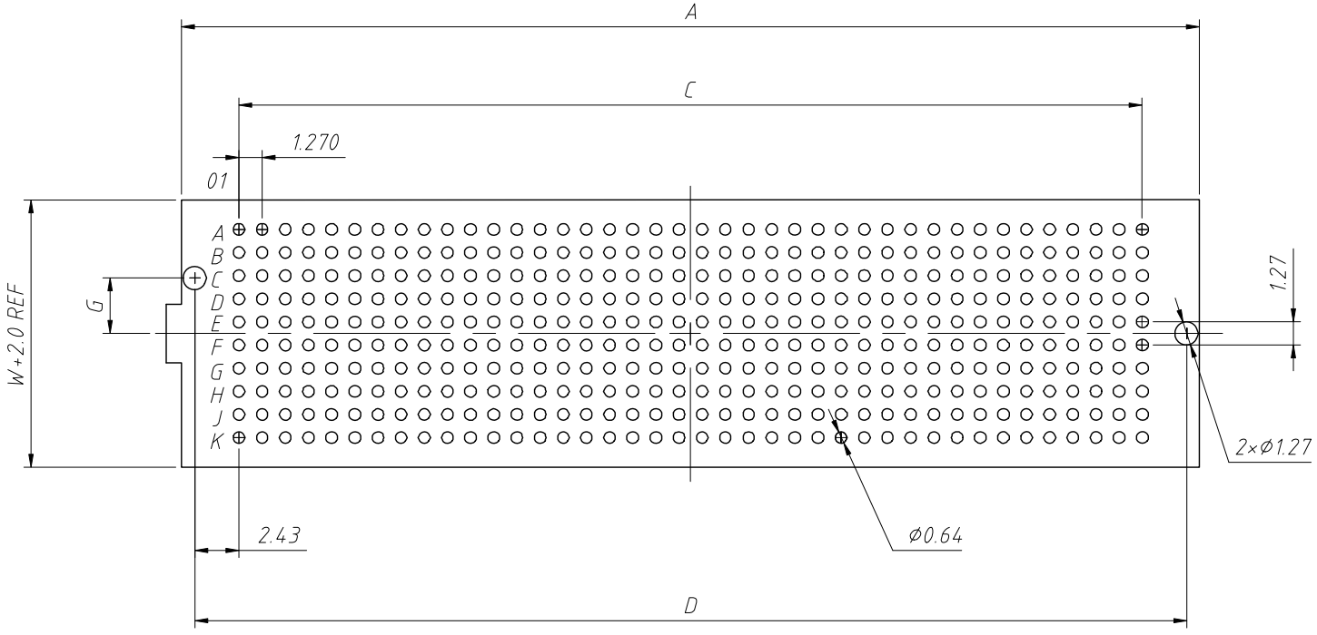
Recommended PC Board Pattern Top View
