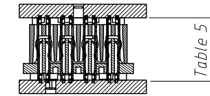
Mating Height Dimension
