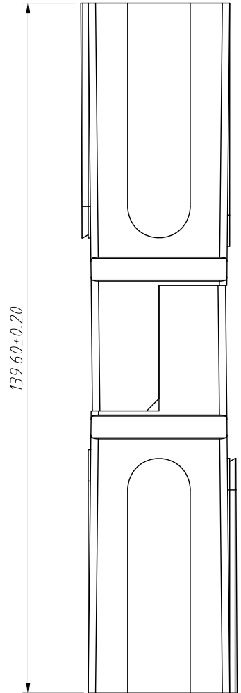
Mating Dimensions
