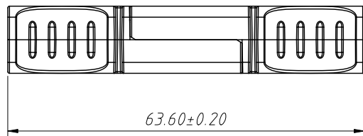
Mating Dimensions
