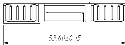
Mating Dimensions
