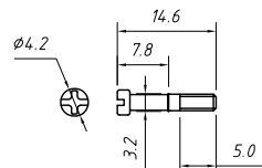
Short screw
