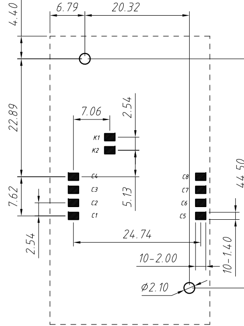
RECOMMEND PCB LAYOUT (FEMALE) TOLERANCE=±0.05mm
