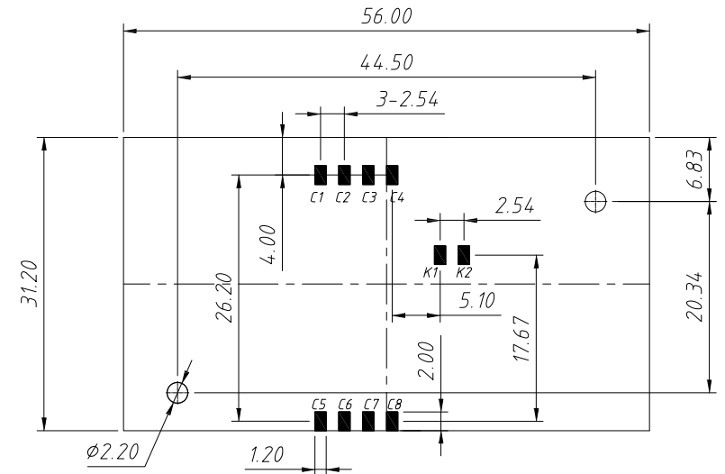
PCB installation diagram
