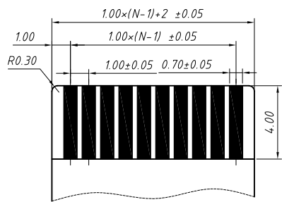
Proper Cable
