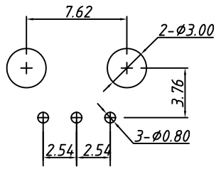
P.C.B LAYOUT TOLERANCE:±0.30
