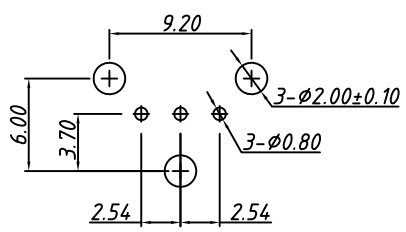
P.C.B LAYOUT TOLERANCE:±0.30
