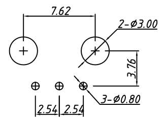
P.C.B LAYOUT TOLERANCE:±0.30
