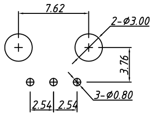
P.C.B LAYOUT TOLERANCE:±0.30
