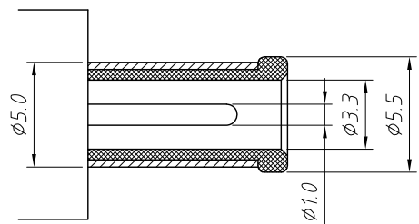
DC MATE PLUG
