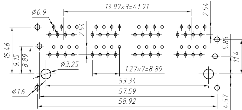
PCB Layout
