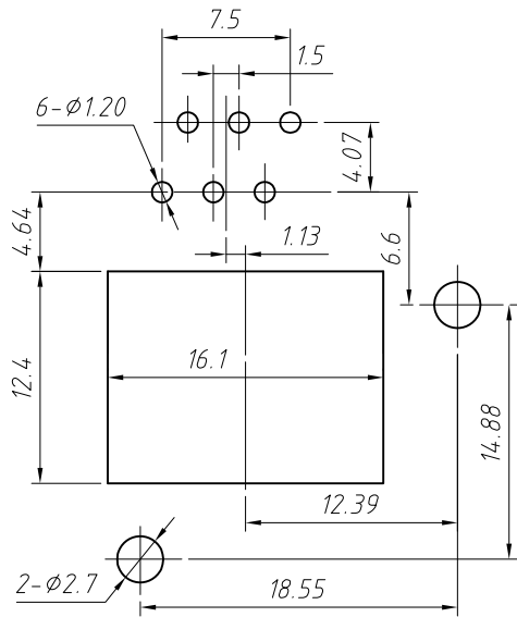
PCB Layout
