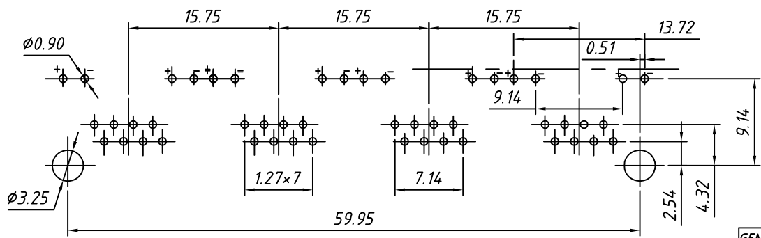
PCB Layout
