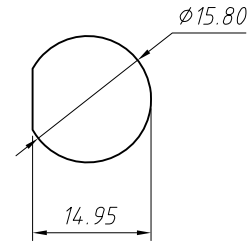
Mounting Hole Dimensions
