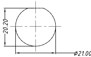
PANEL CUT-OUT Thickness 3.0mm Max
