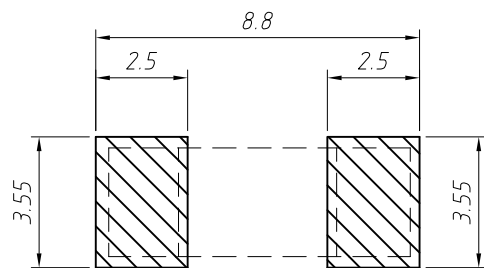
Board Layout
