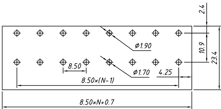
PCB LAYOUT
