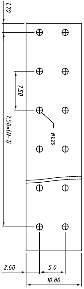
PCB LAYOUT
