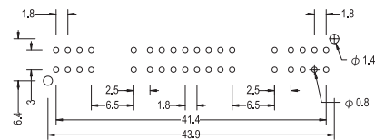
P.C.B. HOLE DETAIL
