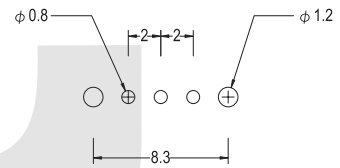
P.C.B. HOLE DETAIL
