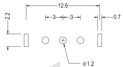
P.C.B. HOLE DETAIL
